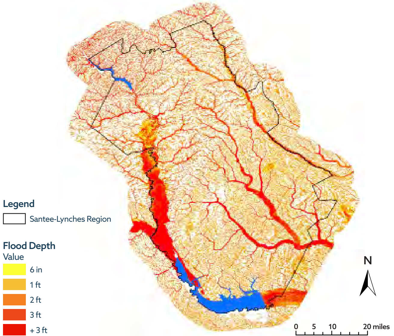
Figure 3.3 Flood Depth
