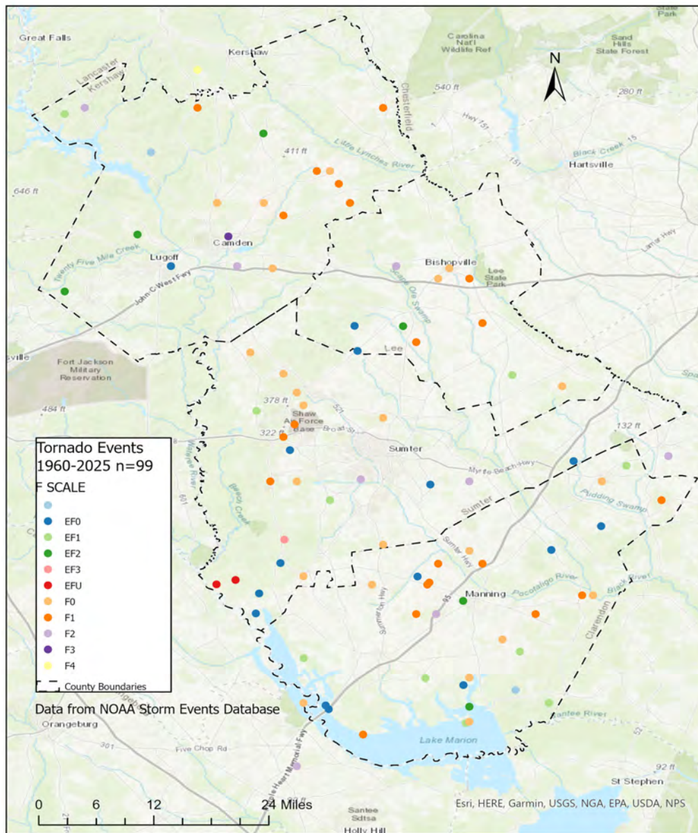
Figure 3.10 Tornado Events
