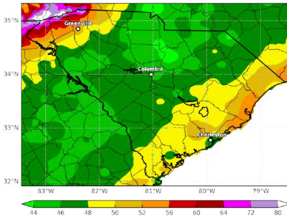
Figure 3.1 SC Average Annual Precipitation (inches)
